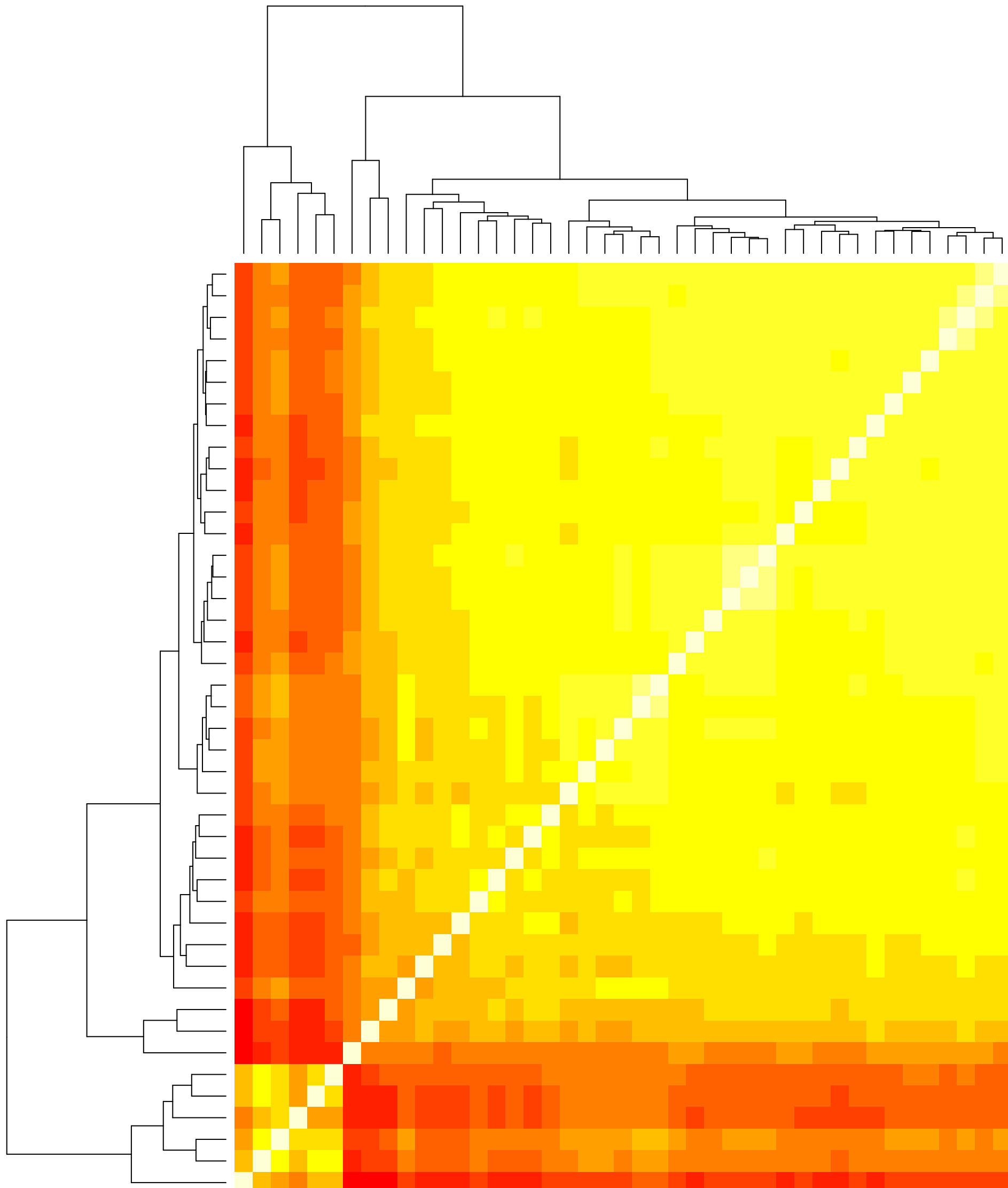
Clustering by samples for: Open_Chromatin (yellow: high, red: low)
