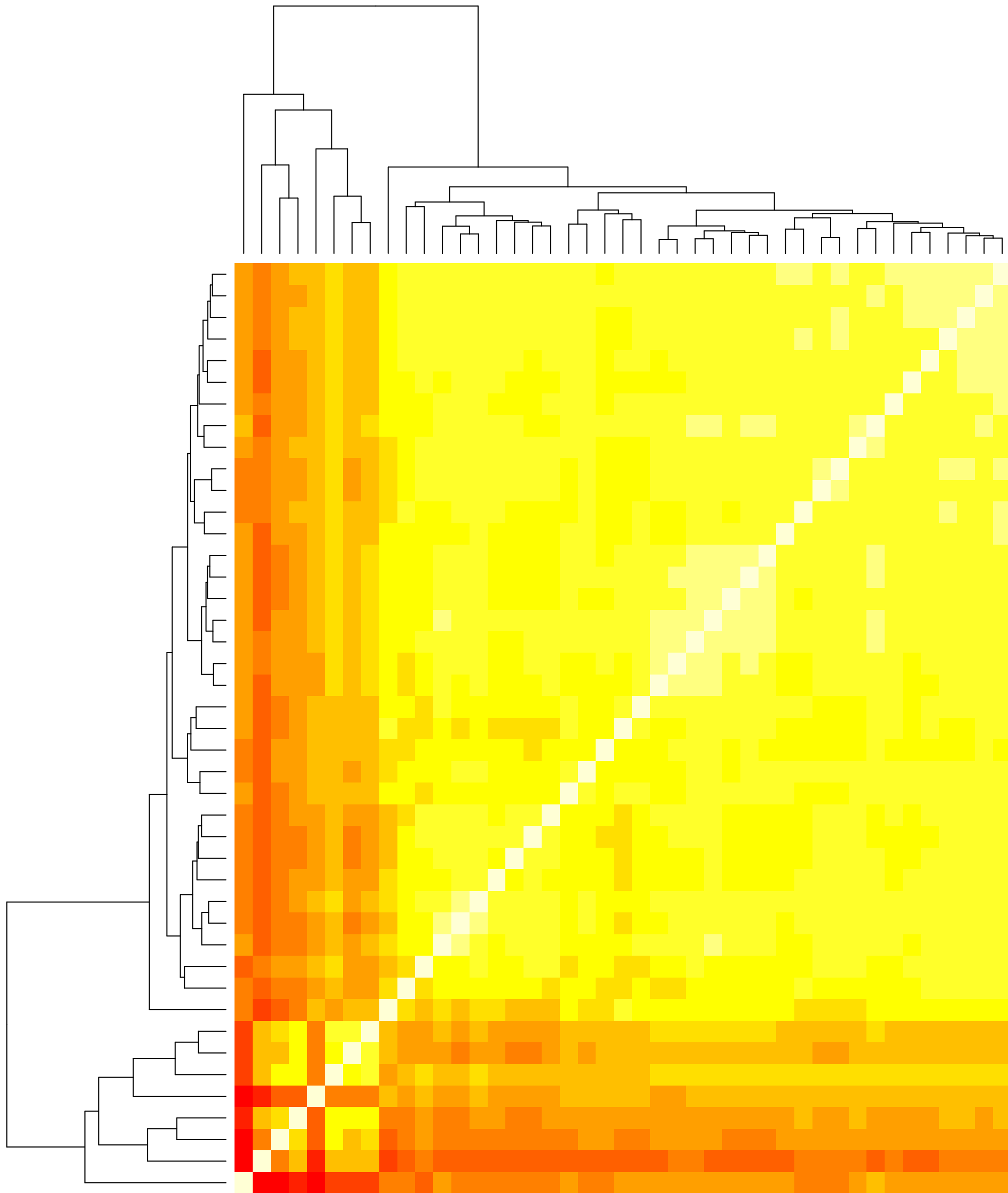
Clustering by samples for: Promoter_region (yellow: high, red: low)
