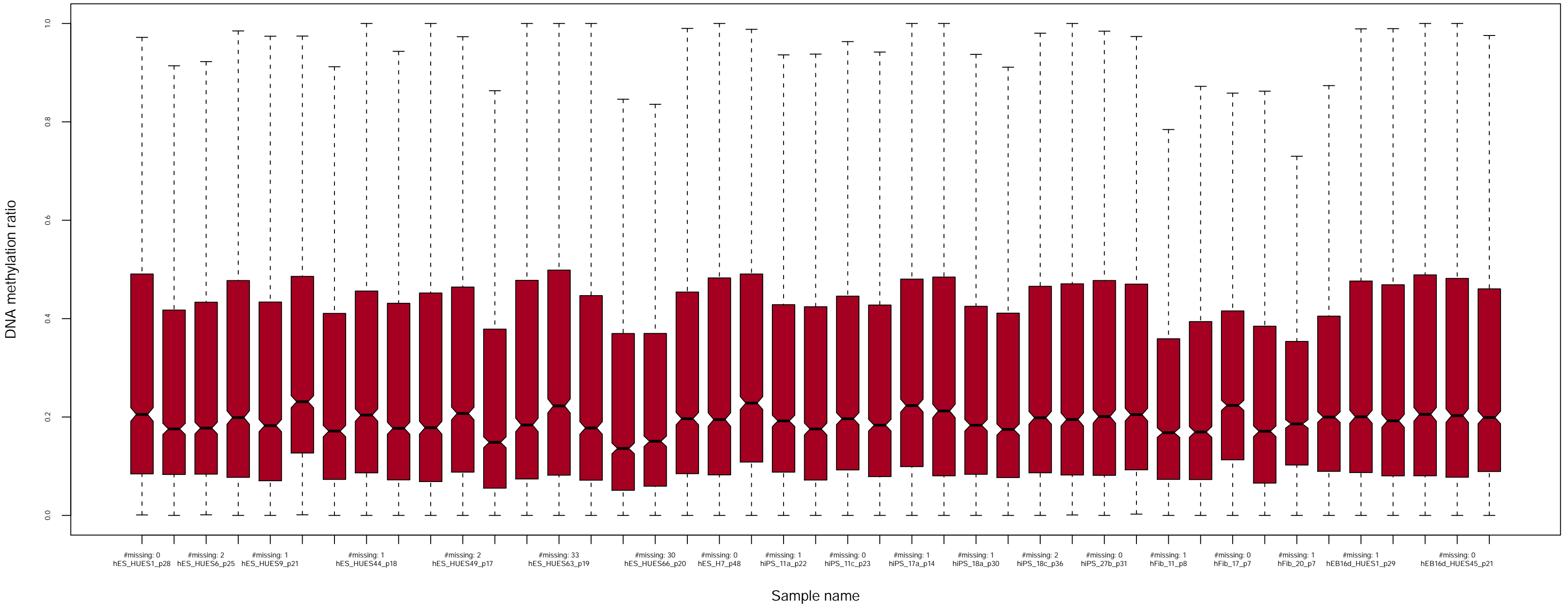
CellStateGene_Promoter (#regions: 2124) – Mean DNA methylation levels
